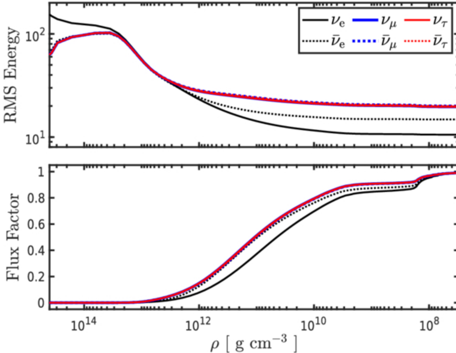
Figure 16. from Eirik Endeve et al 2026 Astrophys. J. Suppl. 284 doi:10.3847/1538-4365/ae57ad https://dx.doi.org/10.3847/1538-4365/ae57ad © 2026. The Author(s). Published by the American Astronomical Society.
