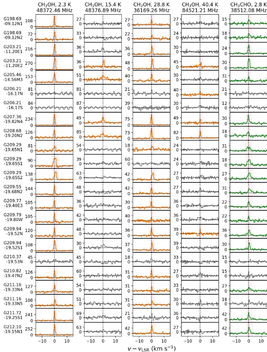
Figure C1. Molecular spectra from Shih-Ying Hsu et al 2026 Astrophys. J. Suppl. 284 doi:10.3847/1538-4365/ae579b https://dx.doi.org/10.3847/1538-4365/ae579b © 2026. The Author(s). Published by the American Astronomical Society.
