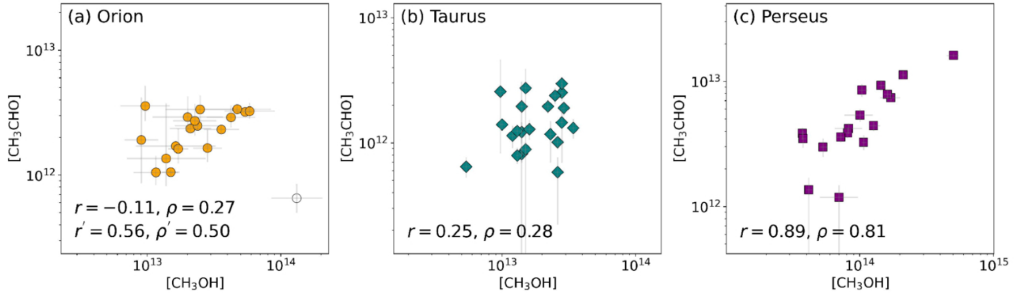
Figure 4. from Shih-Ying Hsu et al 2026 Astrophys. J. Suppl. 284 doi:10.3847/1538-4365/ae579b https://dx.doi.org/10.3847/1538-4365/ae579b © 2026. The Author(s). Published by the American Astronomical Society.
