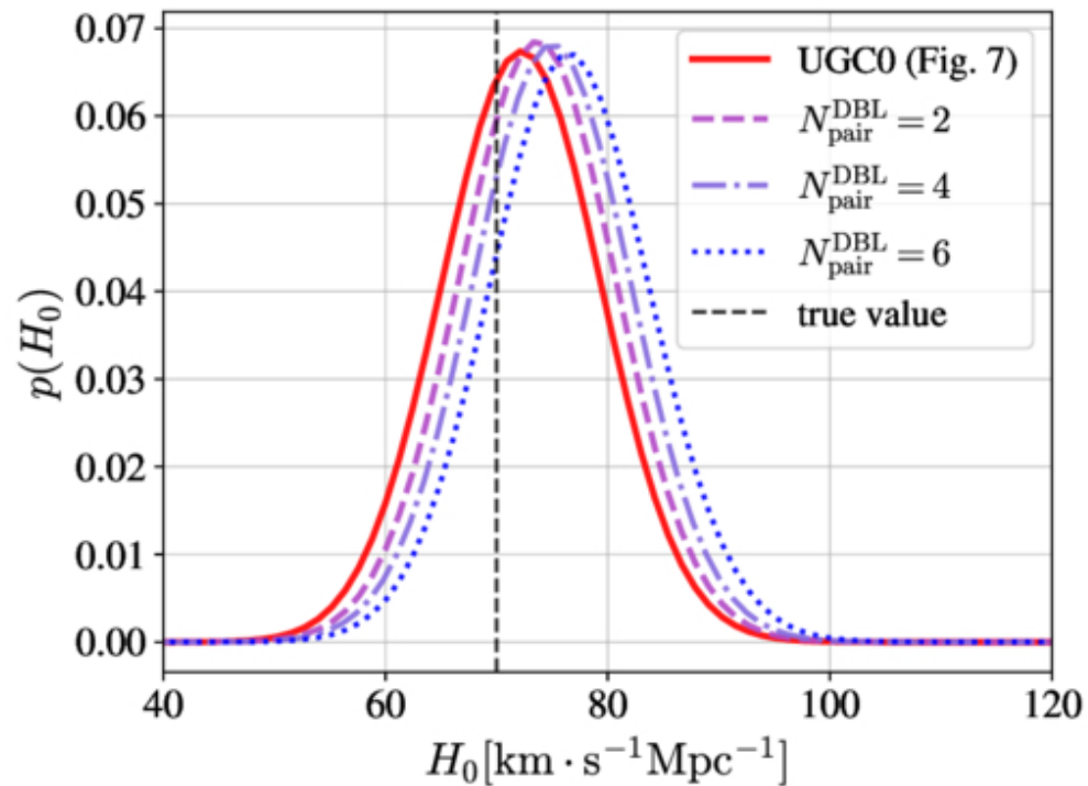
(a) H_0 inferred from an unlensed population containing hidden unlensed signals
