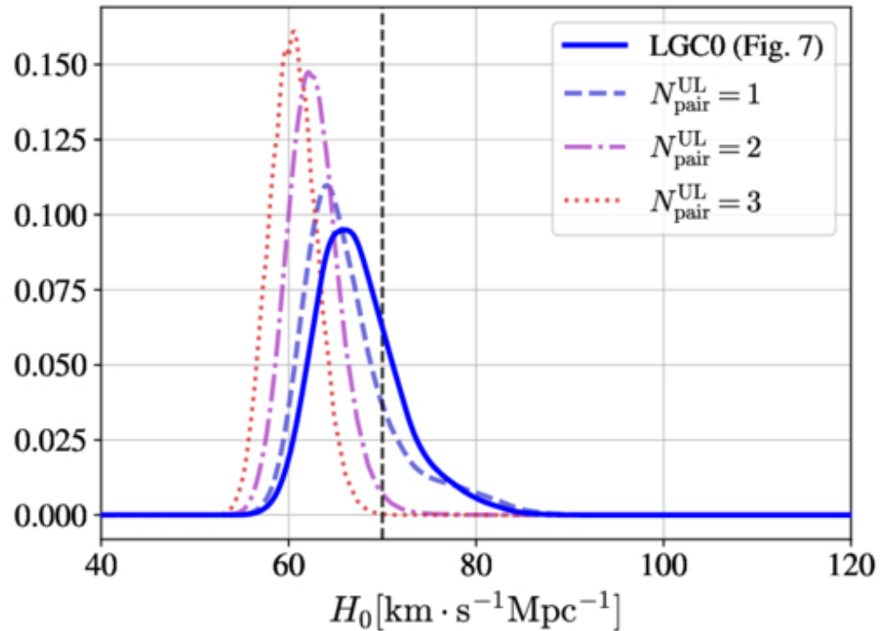
(b) H_0 inferred from a lensed population containing hidden unlensed signals
