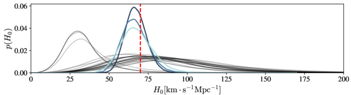
(c) Delensing with SIE model
