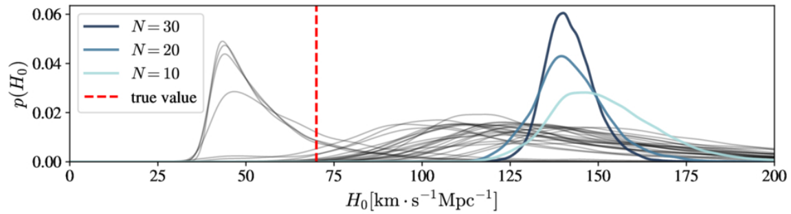
Figure 8. from Eungwang Seo et al 2026 Astrophys. J. Suppl. 284 doi:10.3847/1538-4365/ae579a https://dx.doi.org/10.3847/1538-4365/ae579a © 2026. The Author(s). Published by the American Astronomical Society.
