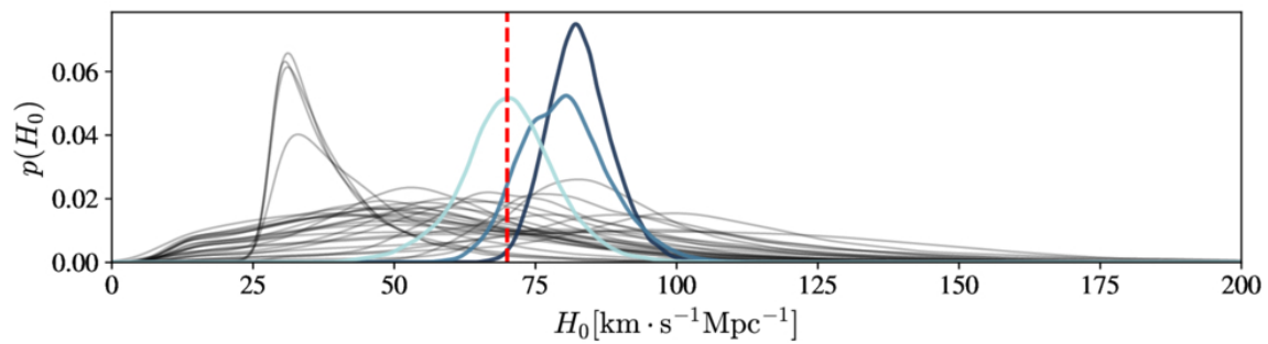
(b) Delensing with SIS model
