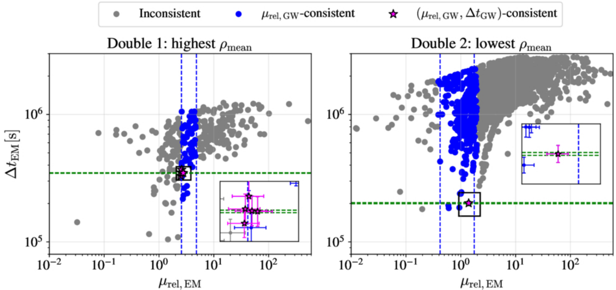
Figure 3. from Eungwang Seo et al 2026 Astrophys. J. Suppl. 284 doi:10.3847/1538-4365/ae579a https://dx.doi.org/10.3847/1538-4365/ae579a © 2026. The Author(s). Published by the American Astronomical Society.
