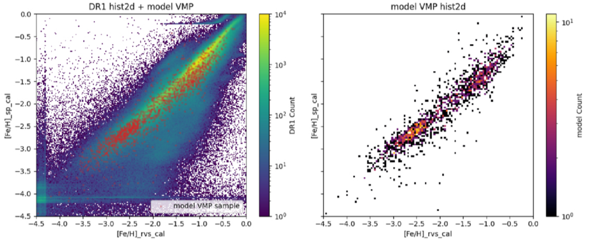
Figure 9. from Chen Yang et al 2026 Astrophys. J. Suppl. 284 doi:10.3847/1538-4365/ae578a https://dx.doi.org/10.3847/1538-4365/ae578a © 2026. The Author(s). Published by the American Astronomical Society.
