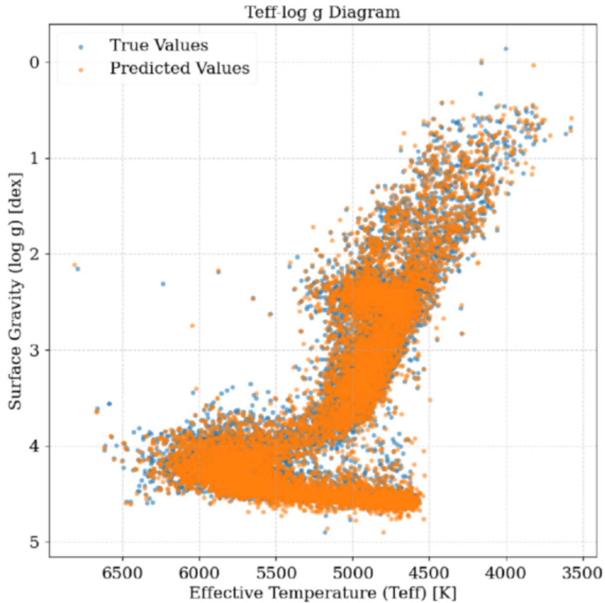
Figure 6. from Chen Yang et al 2026 Astrophys. J. Suppl. 284 doi:10.3847/1538-4365/ae578a https://dx.doi.org/10.3847/1538-4365/ae578a © 2026. The Author(s). Published by the American Astronomical Society.
