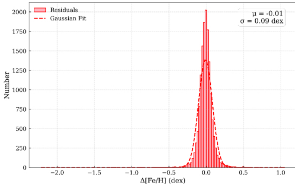
(a) Residual distribution of [\text{Fe}/\text{H}] .
