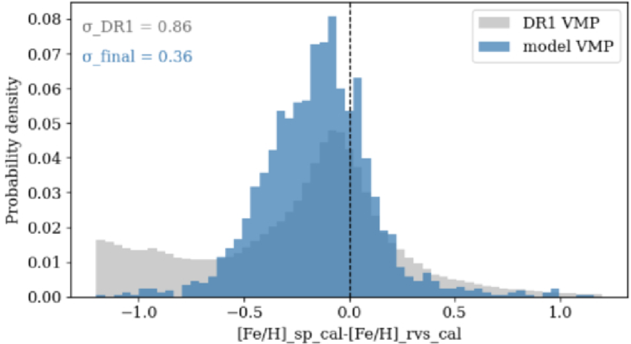
Figure 10. from Chen Yang et al 2026 Astrophys. J. Suppl. 284 doi:10.3847/1538-4365/ae578a https://dx.doi.org/10.3847/1538-4365/ae578a © 2026. The Author(s). Published by the American Astronomical Society.
