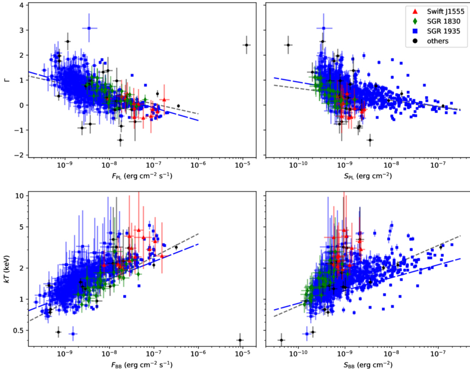
Figure 9. from Che-Yen Chu et al 2026 Astrophys. J. Suppl. 284 doi:10.3847/1538-4365/ae5655 https://dx.doi.org/10.3847/1538-4365/ae5655 © 2026. The Author(s). Published by the American Astronomical Society.
