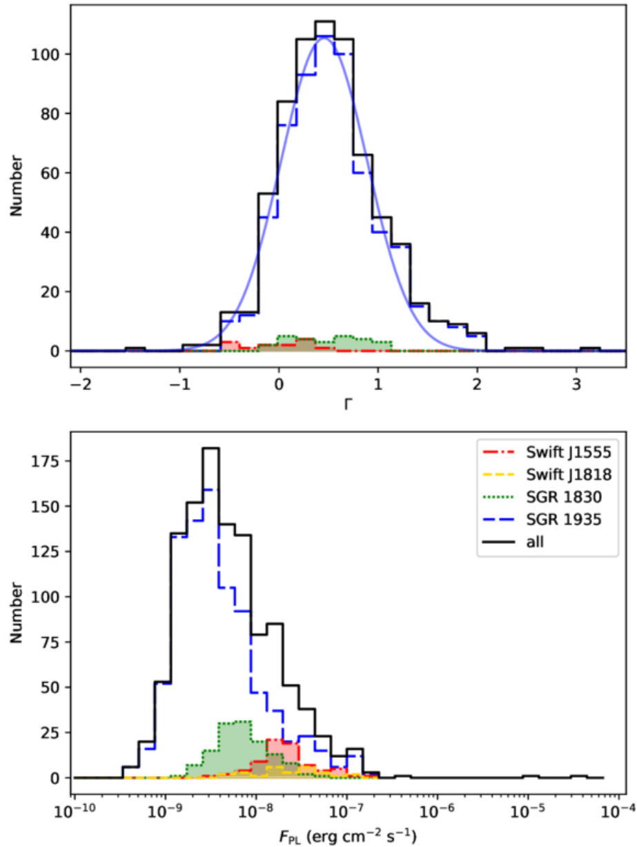
Figure 5. from Che-Yen Chu et al 2026 Astrophys. J. Suppl. 284 doi:10.3847/1538-4365/ae5655 https://dx.doi.org/10.3847/1538-4365/ae5655 © 2026. The Author(s). Published by the American Astronomical Society.
