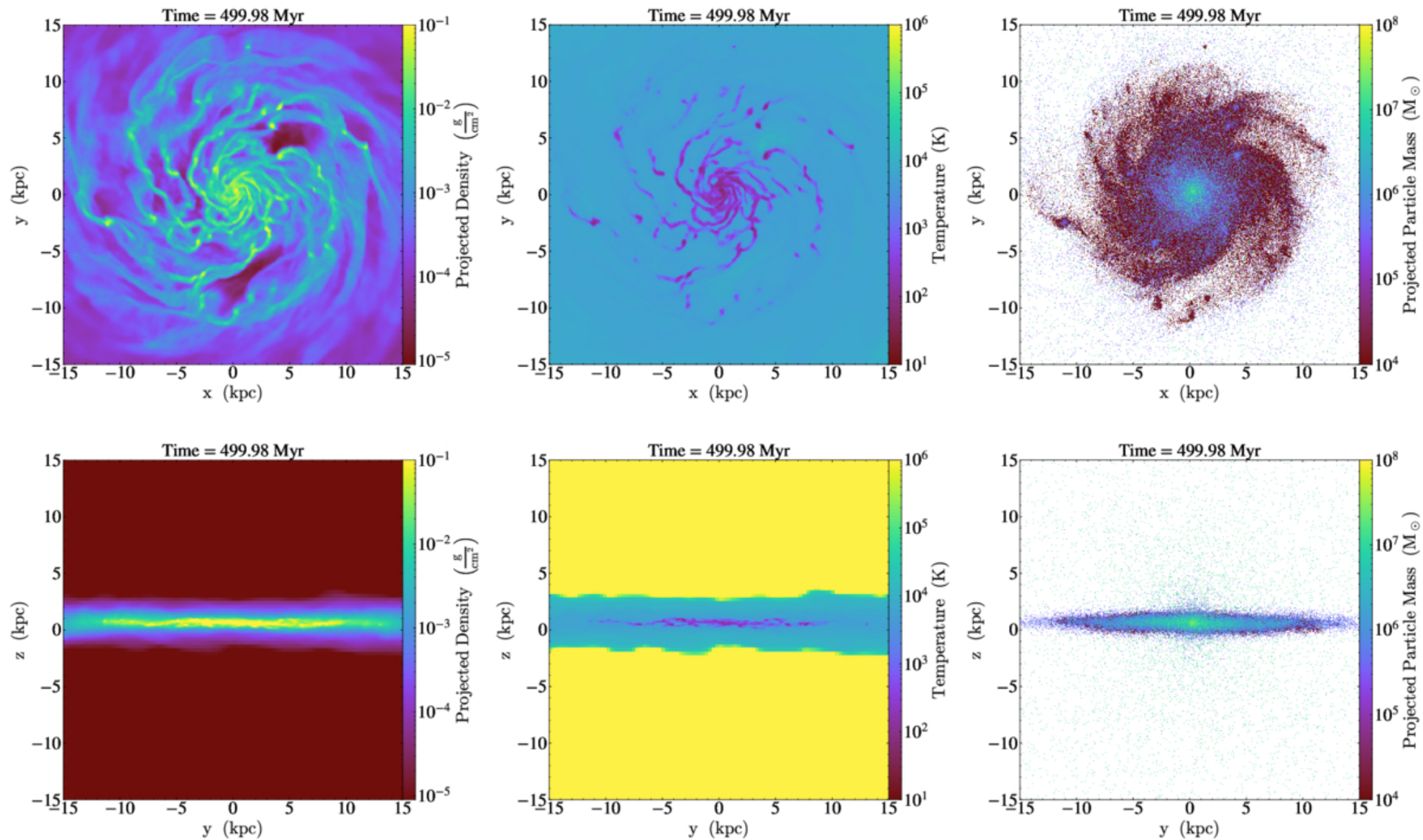
Figure 9. from Shin-Rong Tsai et al 2026 Astrophys. J. Suppl. 284 doi:10.3847/1538-4365/ae5640 https://dx.doi.org/10.3847/1538-4365/ae5640 © 2026. The Author(s). Published by the American Astronomical Society.
