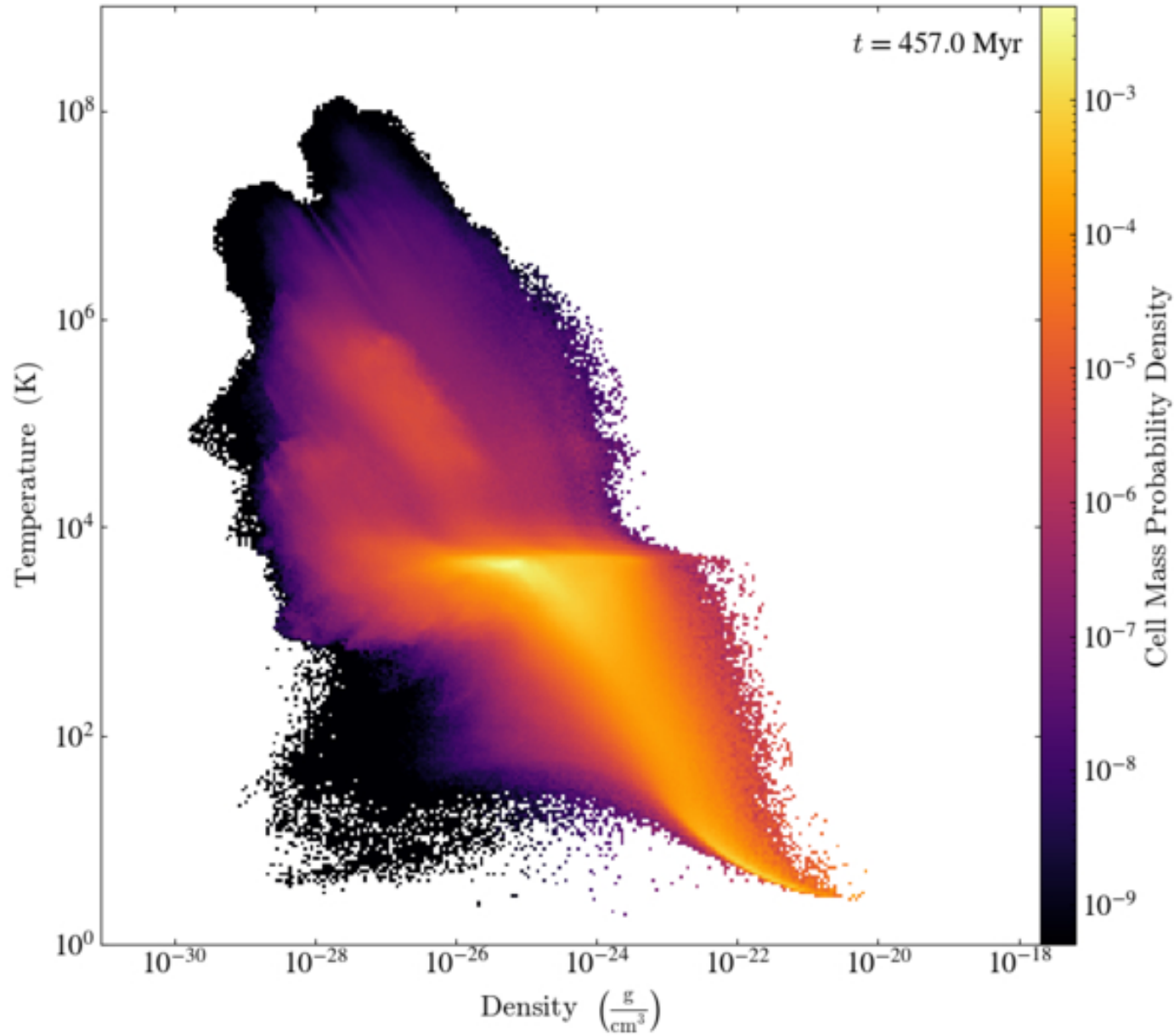
Figure 5. from Shin-Rong Tsai et al 2026 Astrophys. J. Suppl. 284 doi:10.3847/1538-4365/ae5640 https://dx.doi.org/10.3847/1538-4365/ae5640 © 2026. The Author(s). Published by the American Astronomical Society.
