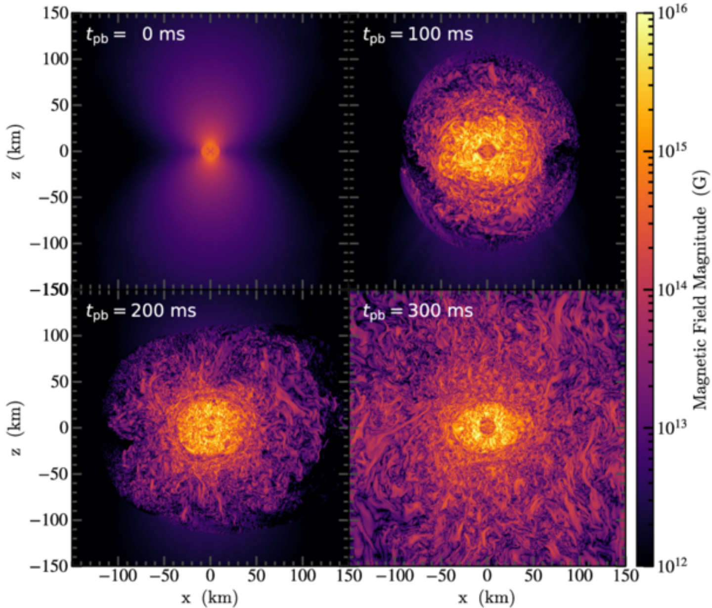
Figure 3. from Shin-Rong Tsai et al 2026 Astrophys. J. Suppl. 284 doi:10.3847/1538-4365/ae5640 https://dx.doi.org/10.3847/1538-4365/ae5640 © 2026. The Author(s). Published by the American Astronomical Society.
