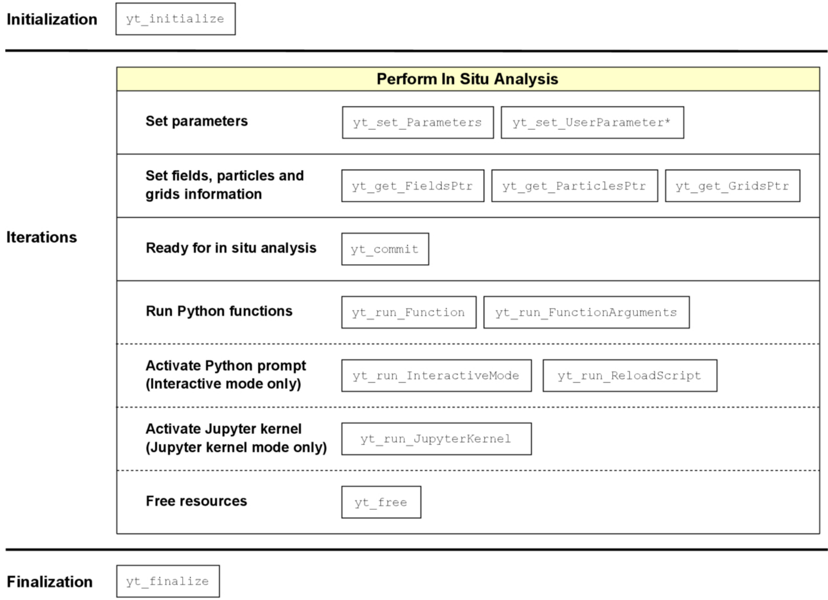
Figure 2. from Shin-Rong Tsai et al 2026 Astrophys. J. Suppl. 284 doi:10.3847/1538-4365/ae5640 https://dx.doi.org/10.3847/1538-4365/ae5640 © 2026. The Author(s). Published by the American Astronomical Society.
