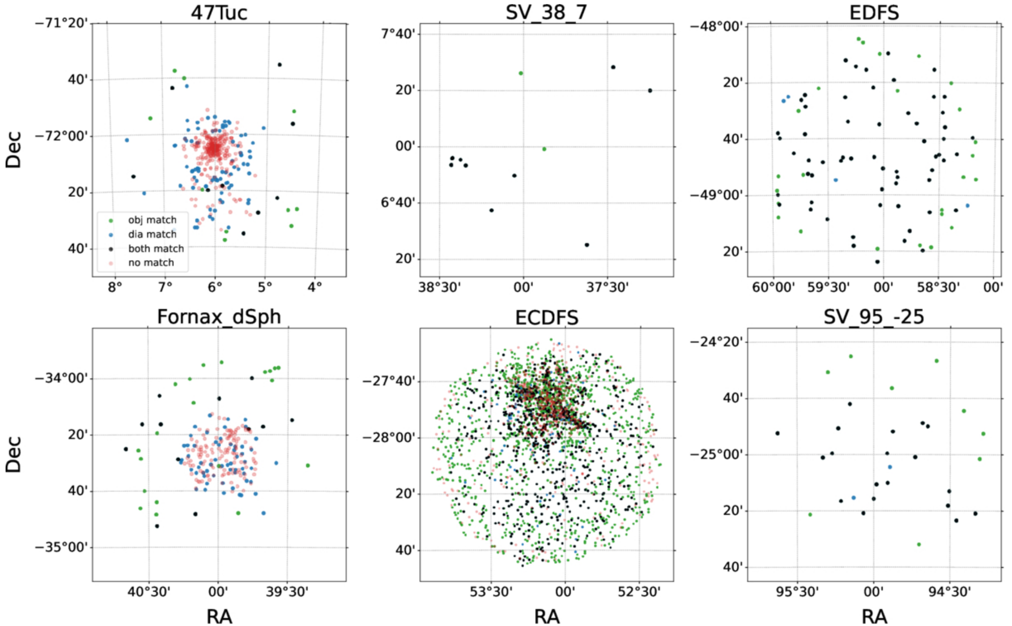
Figure 3. from Yuankun David Wang et al 2026 Astrophys. J. Suppl. 284 doi:10.3847/1538-4365/ae5247 https://dx.doi.org/10.3847/1538-4365/ae5247 © 2026. The Author(s). Published by the American Astronomical Society.
