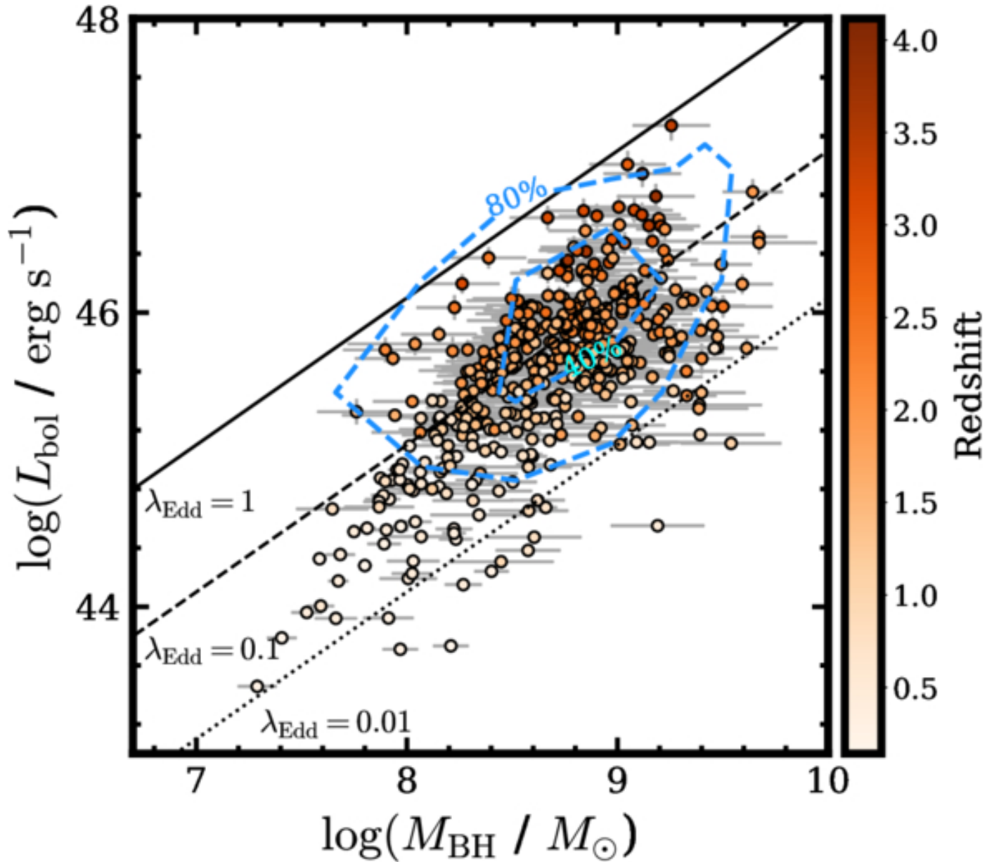
Figure 4. from Dohyeong Kim et al 2026 Astrophys. J. Suppl. 284 doi:10.3847/1538-4365/ae5245 https://dx.doi.org/10.3847/1538-4365/ae5245 © 2026. The Author(s). Published by the American Astronomical Society.
