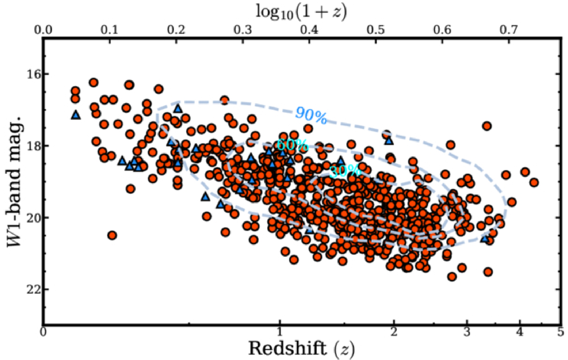
Figure 1. from Dohyeong Kim et al 2026 Astrophys. J. Suppl. 284 doi:10.3847/1538-4365/ae5245 https://dx.doi.org/10.3847/1538-4365/ae5245 © 2026. The Author(s). Published by the American Astronomical Society.
