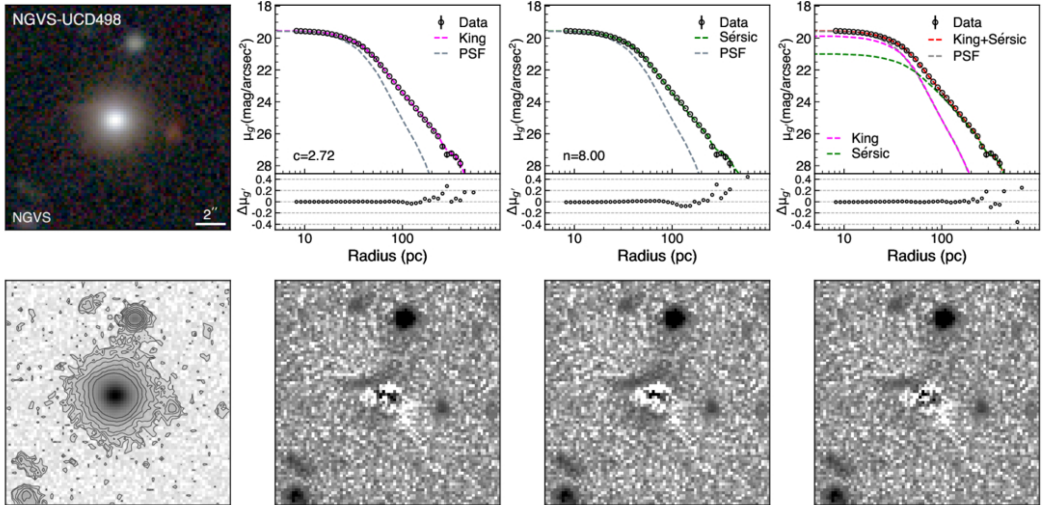
Figure 3. from Kaixiang Wang et al 2026 Astrophys. J. Suppl. 285 doi:10.3847/1538-4365/ae5231 https://dx.doi.org/10.3847/1538-4365/ae5231 © 2026. The Author(s). Published by the American Astronomical Society.
