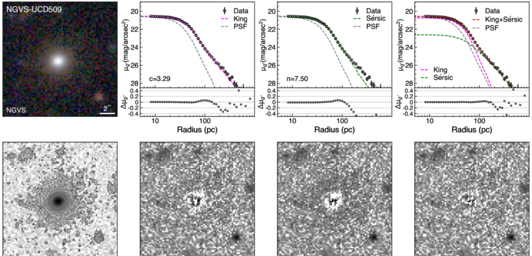
Figure 2. from Kaixiang Wang et al 2026 Astrophys. J. Suppl. 285 doi:10.3847/1538-4365/ae5231 https://dx.doi.org/10.3847/1538-4365/ae5231 © 2026. The Author(s). Published by the American Astronomical Society.
