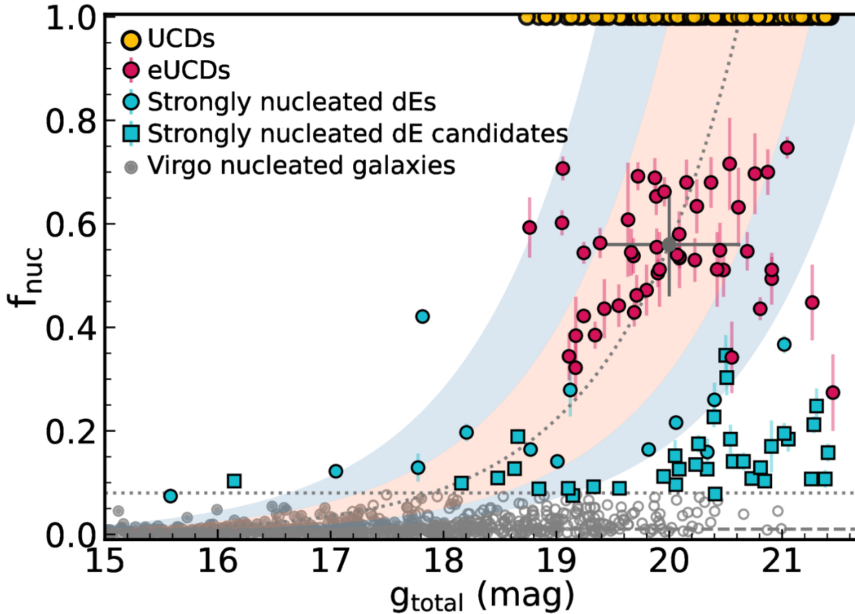
Figure 15. from Kaixiang Wang et al 2026 Astrophys. J. Suppl. 285 doi:10.3847/1538-4365/ae5231 https://dx.doi.org/10.3847/1538-4365/ae5231 © 2026. The Author(s). Published by the American Astronomical Society.
