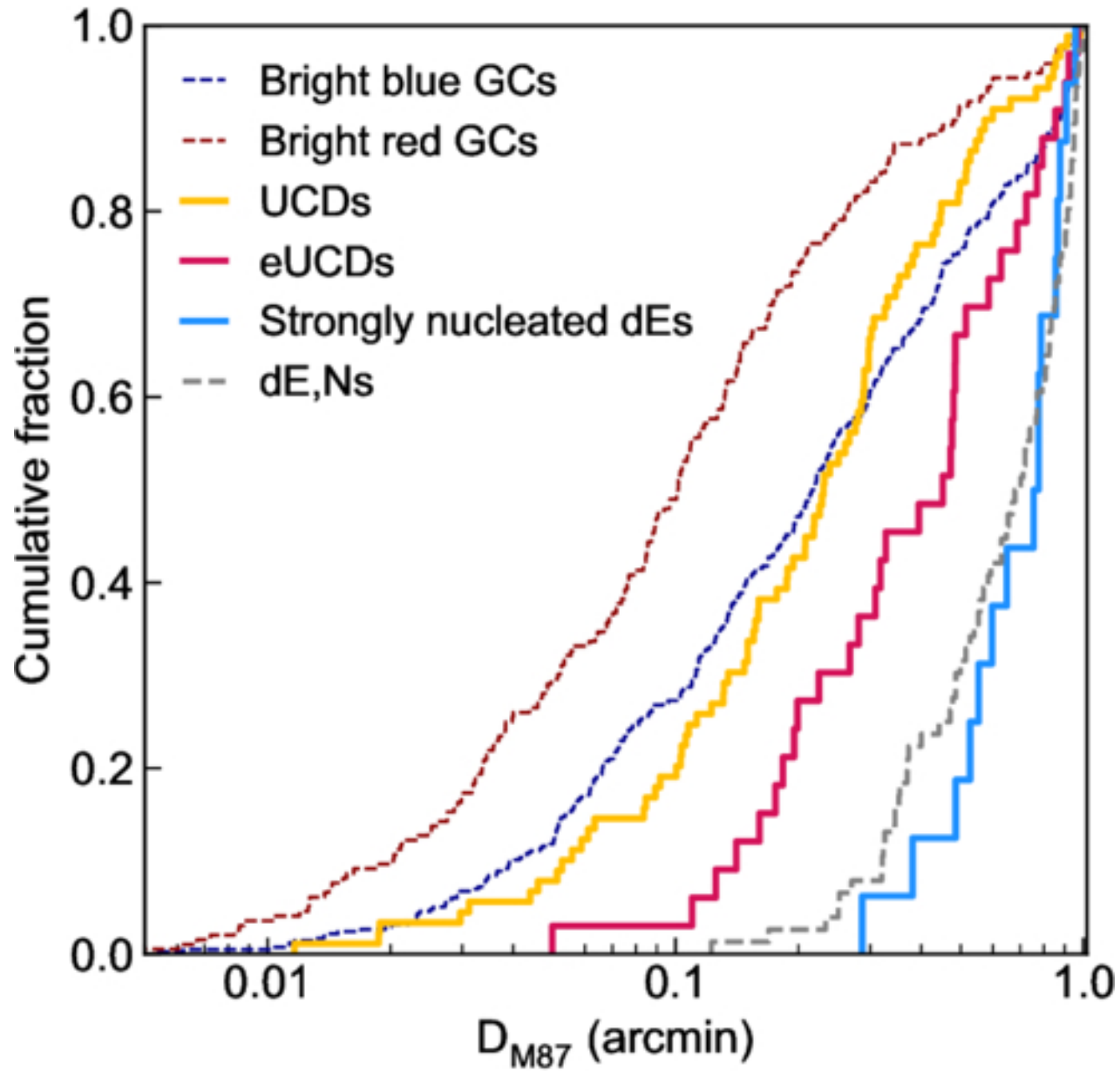
Figure 14. from Kaixiang Wang et al 2026 Astrophys. J. Suppl. 285 doi:10.3847/1538-4365/ae5231 https://dx.doi.org/10.3847/1538-4365/ae5231 © 2026. The Author(s). Published by the American Astronomical Society.
