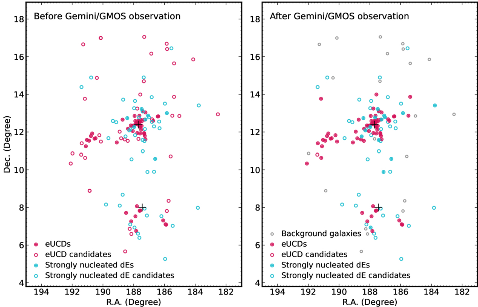
Figure 10. from Kaixiang Wang et al 2026 Astrophys. J. Suppl. 285 doi:10.3847/1538-4365/ae5231 https://dx.doi.org/10.3847/1538-4365/ae5231 © 2026. The Author(s). Published by the American Astronomical Society.
