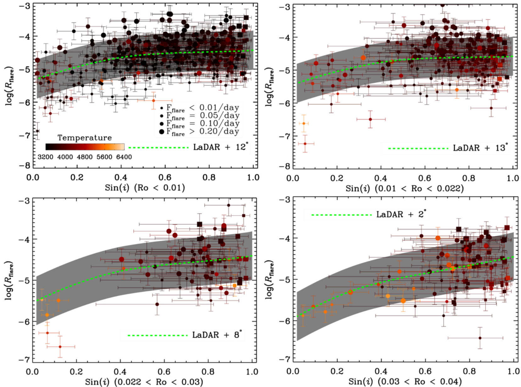
Figure 3. from Huiqin Yang et al 2026 Astrophys. J. Suppl. 283 doi:10.3847/1538-4365/ae50ec https://dx.doi.org/10.3847/1538-4365/ae50ec © 2026. The Author(s). Published by the American Astronomical Society.
