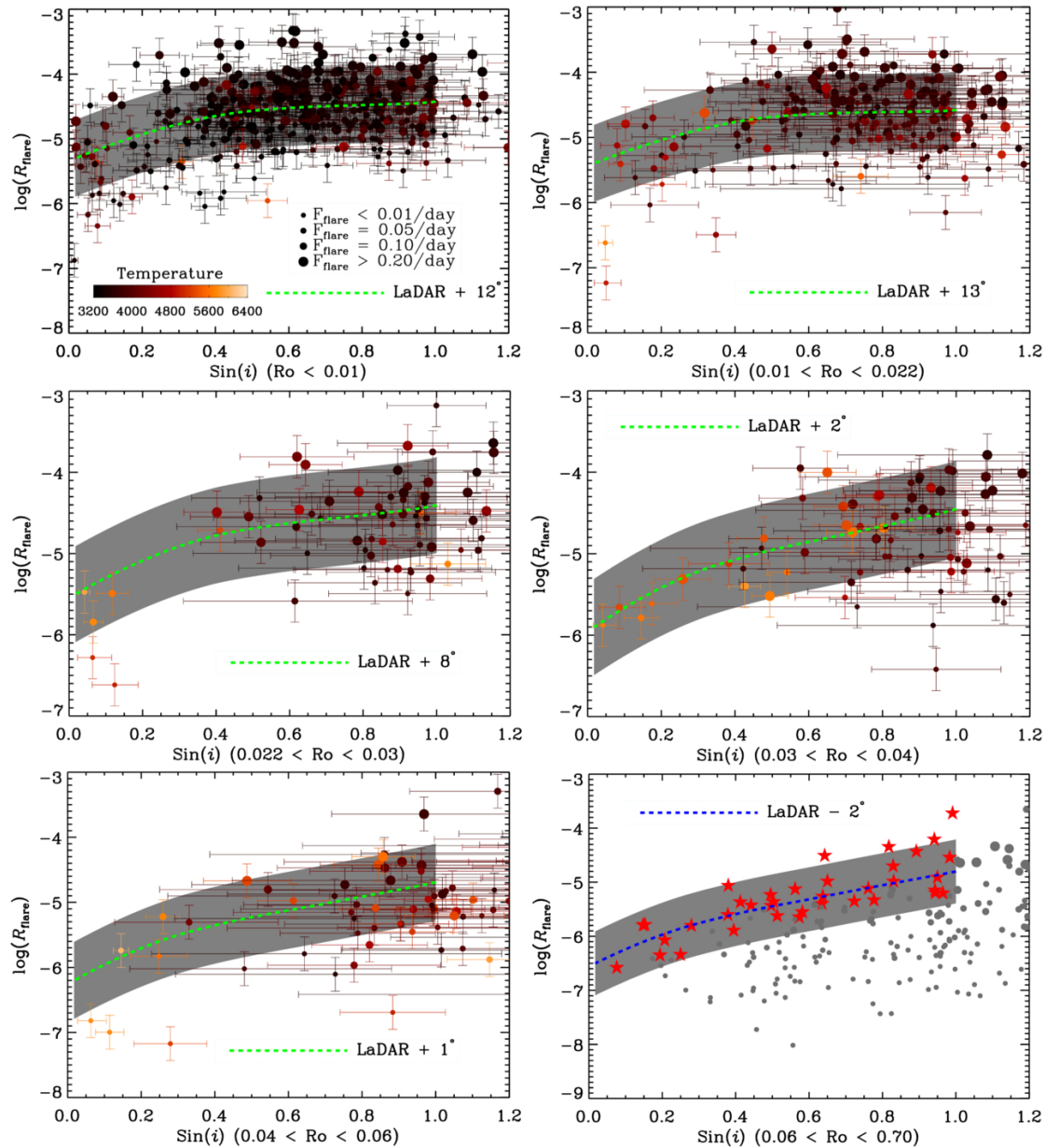
Figure C4. from Huiqin Yang et al 2026 Astrophys. J. Suppl. 283 doi:10.3847/1538-4365/ae50ec https://dx.doi.org/10.3847/1538-4365/ae50ec © 2026. The Author(s). Published by the American Astronomical Society.
