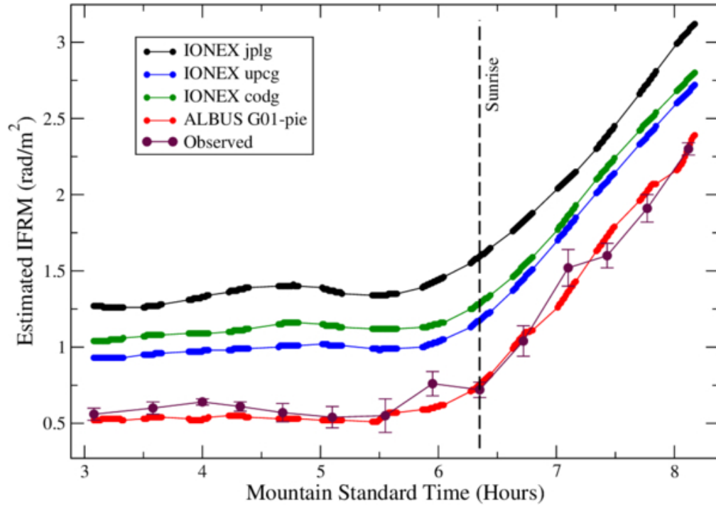
Figure 5. from Richard A. Perley et al 2026 Astrophys. J. Suppl. 283 doi:10.3847/1538-4365/ae503c https://dx.doi.org/10.3847/1538-4365/ae503c © 2026. The Author(s). Published by the American Astronomical Society.
