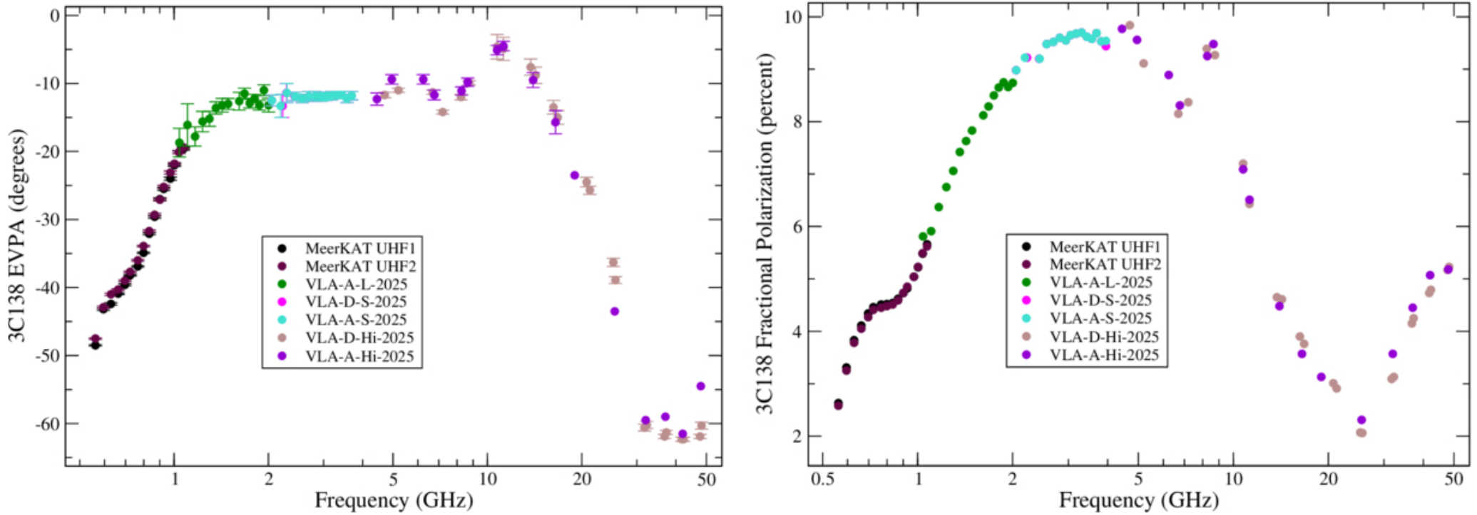
Figure 13. from Richard A. Perley et al 2026 Astrophys. J. Suppl. 283 doi:10.3847/1538-4365/ae503c https://dx.doi.org/10.3847/1538-4365/ae503c © 2026. The Author(s). Published by the American Astronomical Society.
