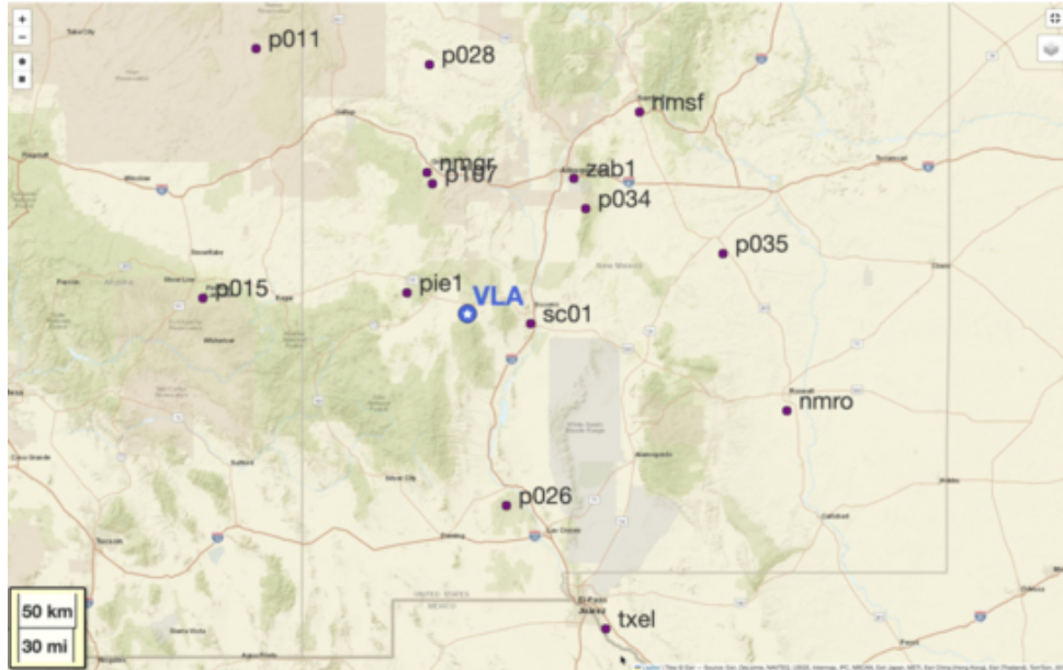
Figure 1. from Richard A. Perley et al 2026 Astrophys. J. Suppl. 283 doi:10.3847/1538-4365/ae503c https://dx.doi.org/10.3847/1538-4365/ae503c © 2026. The Author(s). Published by the American Astronomical Society.
