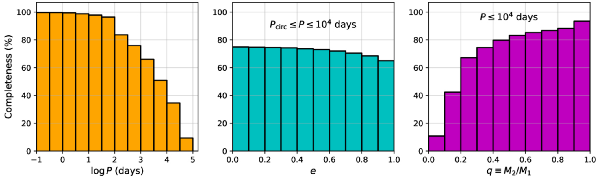
Figure 8. from Guillermo Torres et al 2026 Astrophys. J. Suppl. 283 doi:10.3847/1538-4365/ae4fbb https://dx.doi.org/10.3847/1538-4365/ae4fbb © 2026. The Author(s). Published by the American Astronomical Society.
