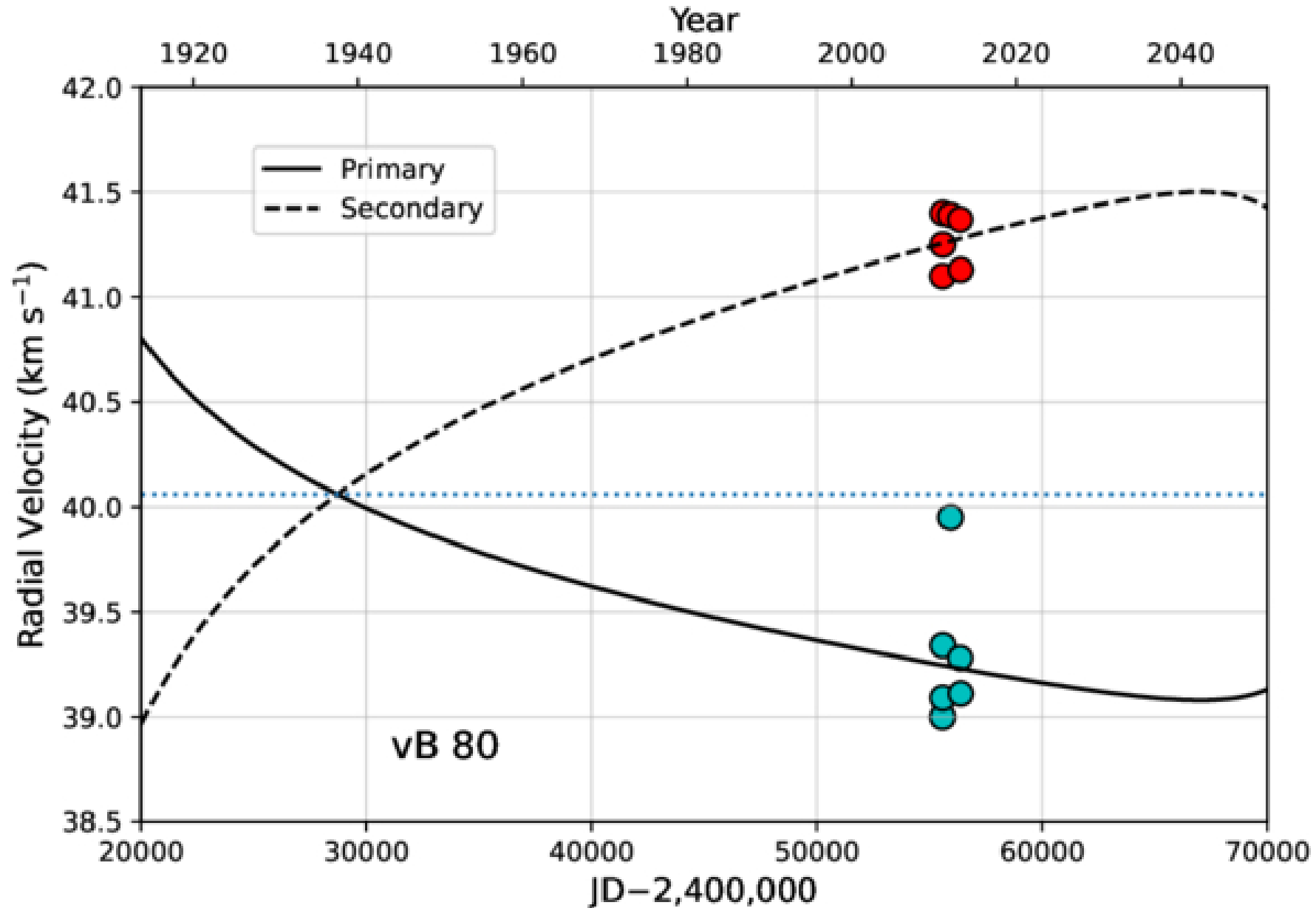
Figure 22. from Guillermo Torres et al 2026 Astrophys. J. Suppl. 283 doi:10.3847/1538-4365/ae4fbb https://dx.doi.org/10.3847/1538-4365/ae4fbb © 2026. The Author(s). Published by the American Astronomical Society.
