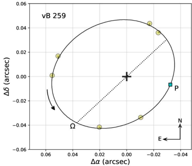
Figure 21. from Guillermo Torres et al 2026 Astrophys. J. Suppl. 283 doi:10.3847/1538-4365/ae4fbb https://dx.doi.org/10.3847/1538-4365/ae4fbb © 2026. The Author(s). Published by the American Astronomical Society.
