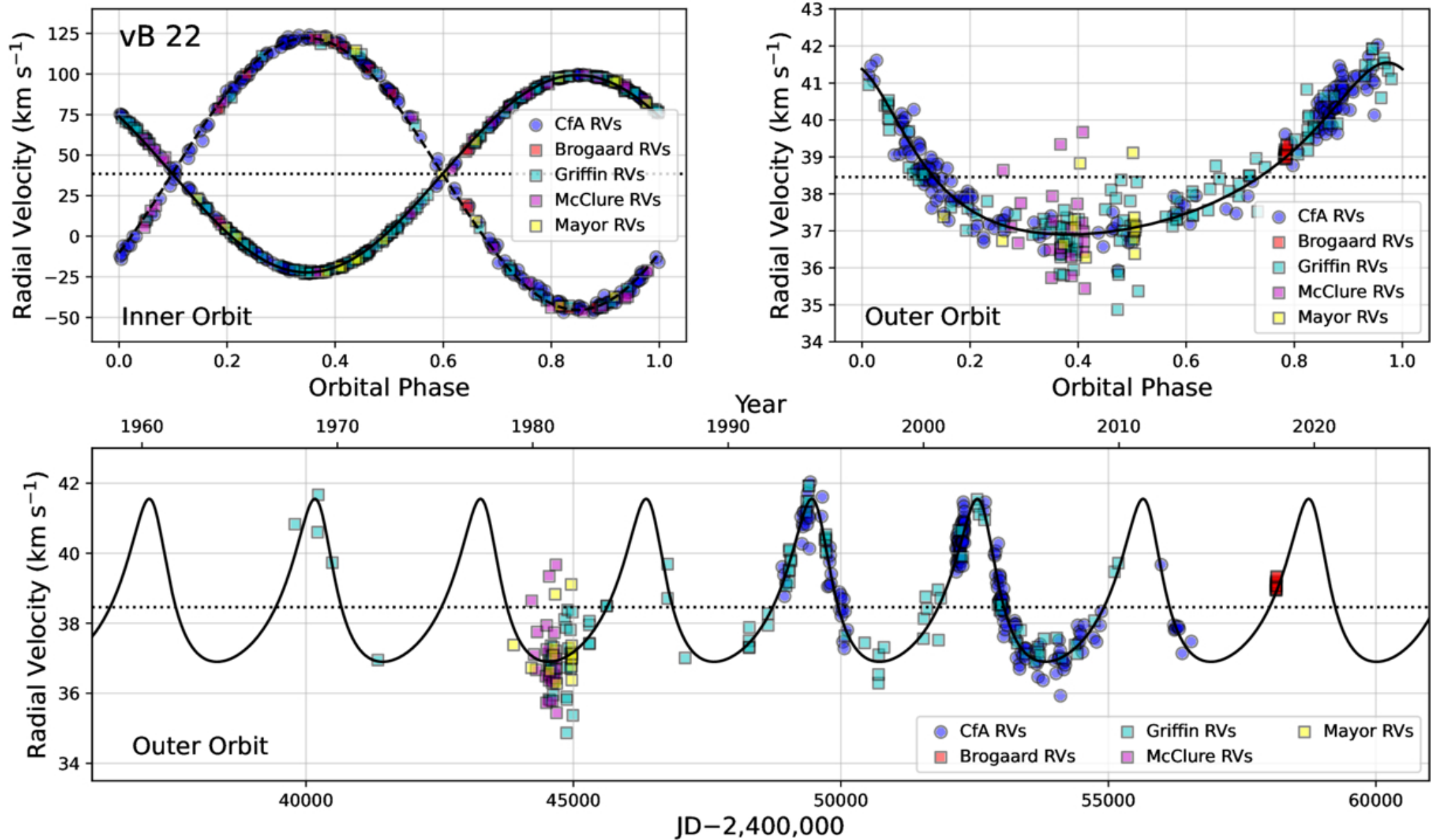
Figure 20. from Guillermo Torres et al 2026 Astrophys. J. Suppl. 283 doi:10.3847/1538-4365/ae4fbb https://dx.doi.org/10.3847/1538-4365/ae4fbb © 2026. The Author(s). Published by the American Astronomical Society.
