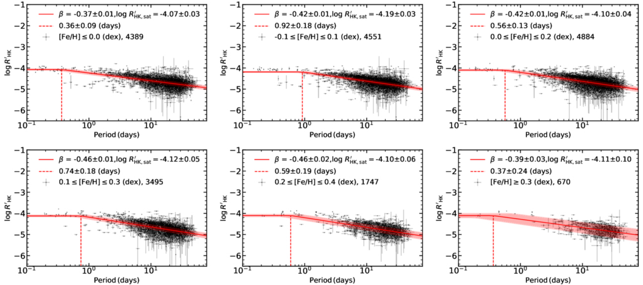
Figure 5. from Weitao Zhang et al 2026 Astrophys. J. Suppl. 283 doi:10.3847/1538-4365/ae4fb2 https://dx.doi.org/10.3847/1538-4365/ae4fb2 © 2026. The Author(s). Published by the American Astronomical Society.
