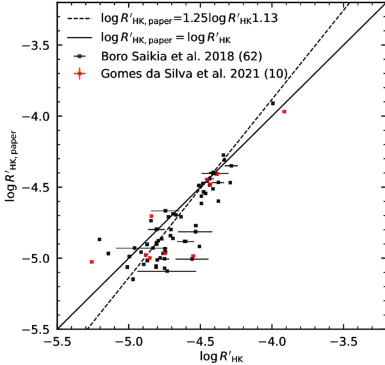
Figure 13. from Weitao Zhang et al 2026 Astrophys. J. Suppl. 283 doi:10.3847/1538-4365/ae4fb2 https://dx.doi.org/10.3847/1538-4365/ae4fb2 © 2026. The Author(s). Published by the American Astronomical Society.
