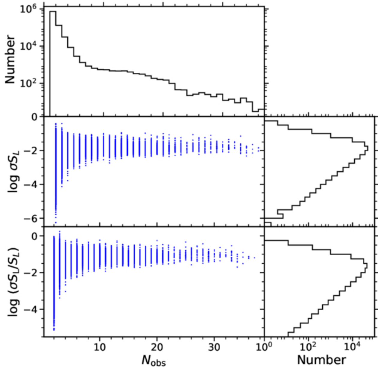
Figure 1. from Weitao Zhang et al 2026 Astrophys. J. Suppl. 283 doi:10.3847/1538-4365/ae4fb2 https://dx.doi.org/10.3847/1538-4365/ae4fb2 © 2026. The Author(s). Published by the American Astronomical Society.
