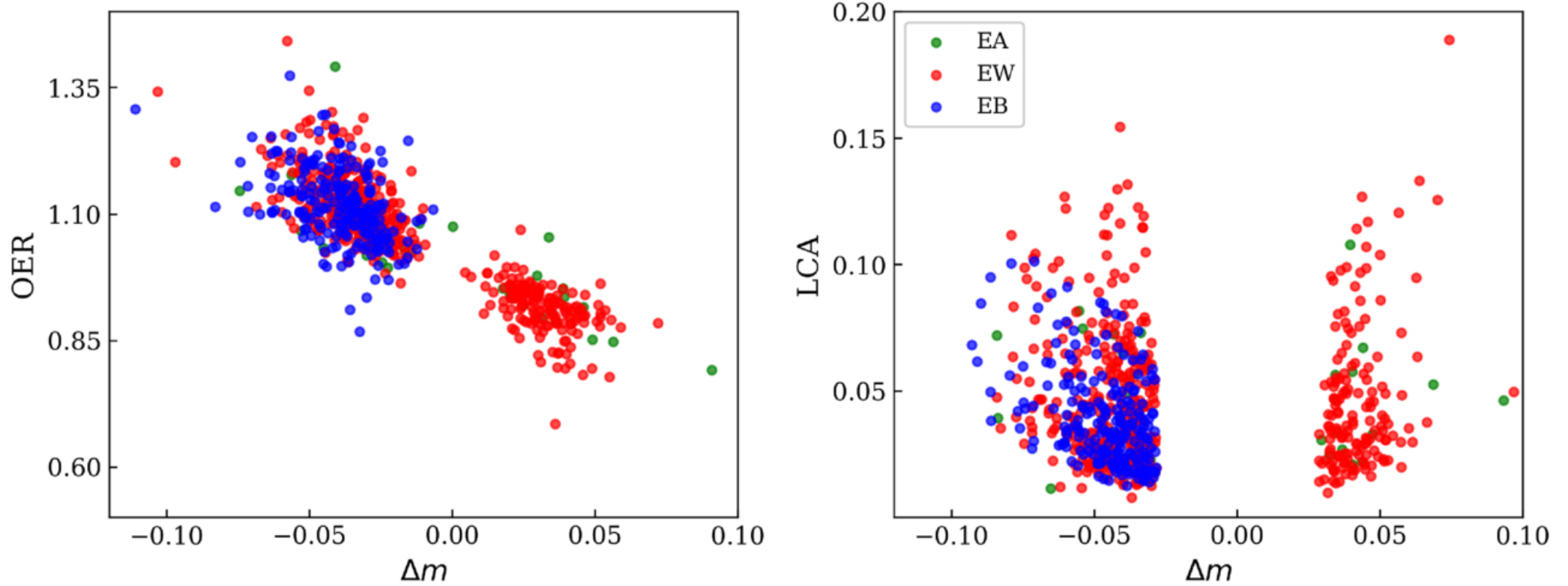
Figure 6. from Jiawen Zhou et al 2026 Astrophys. J. Suppl. 283 doi:10.3847/1538-4365/ae4ed5 https://dx.doi.org/10.3847/1538-4365/ae4ed5 © 2026. The Author(s). Published by the American Astronomical Society.
