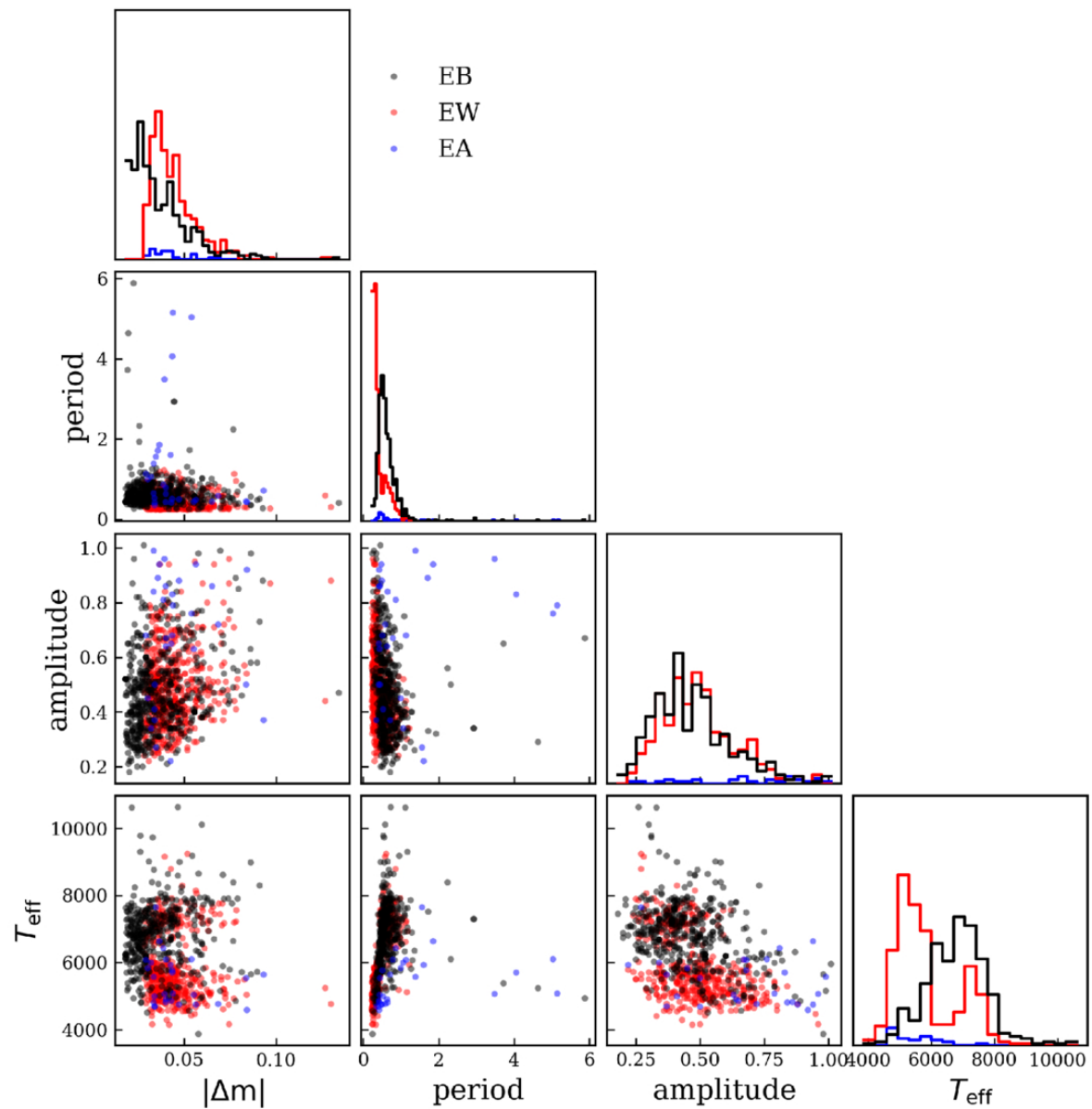
Figure 5. from Jiawen Zhou et al 2026 Astrophys. J. Suppl. 283 doi:10.3847/1538-4365/ae4ed5 https://dx.doi.org/10.3847/1538-4365/ae4ed5 © 2026. The Author(s). Published by the American Astronomical Society.
