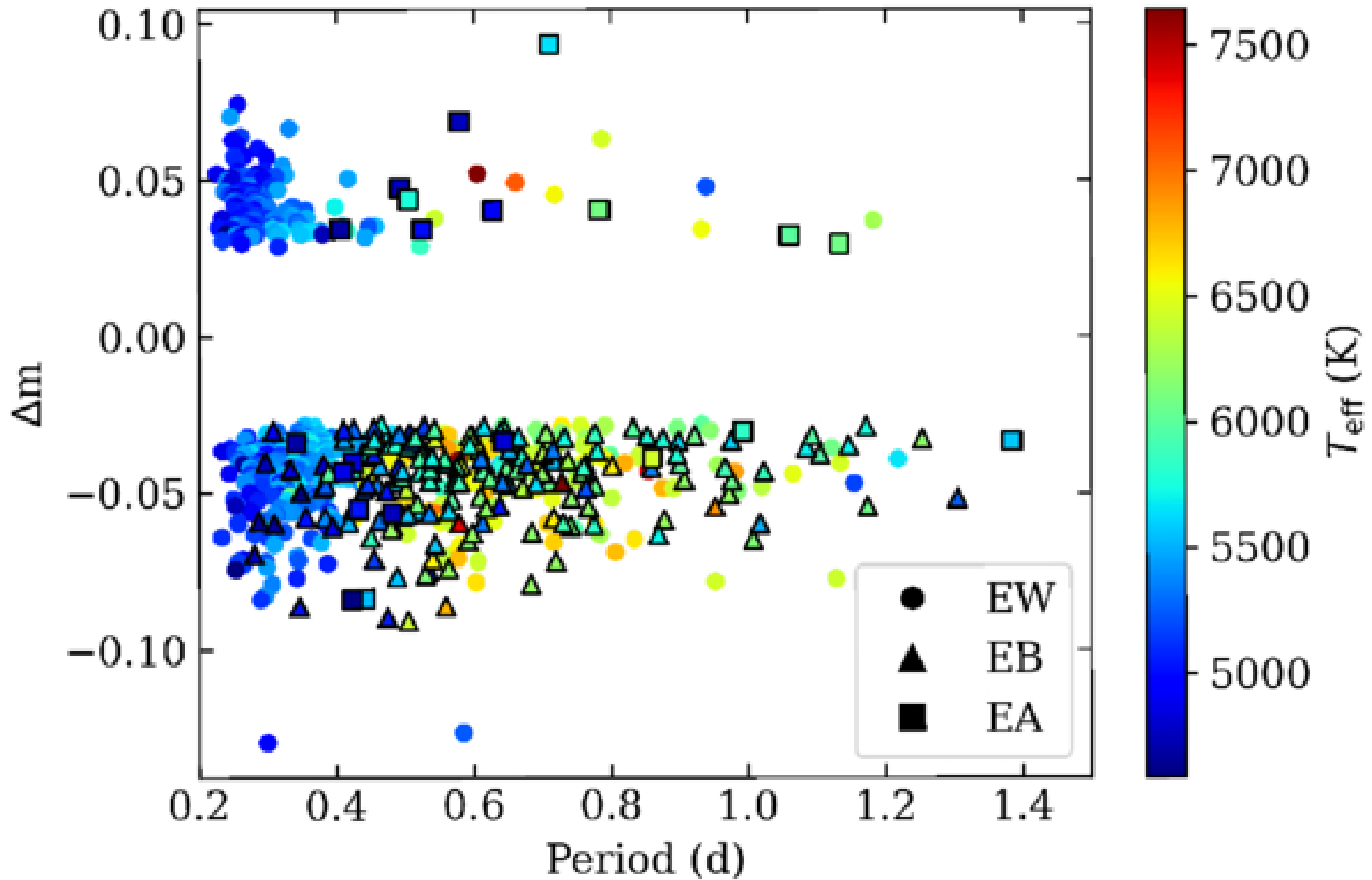
Figure 4. from Jiawen Zhou et al 2026 Astrophys. J. Suppl. 283 doi:10.3847/1538-4365/ae4ed5 https://dx.doi.org/10.3847/1538-4365/ae4ed5 © 2026. The Author(s). Published by the American Astronomical Society.
