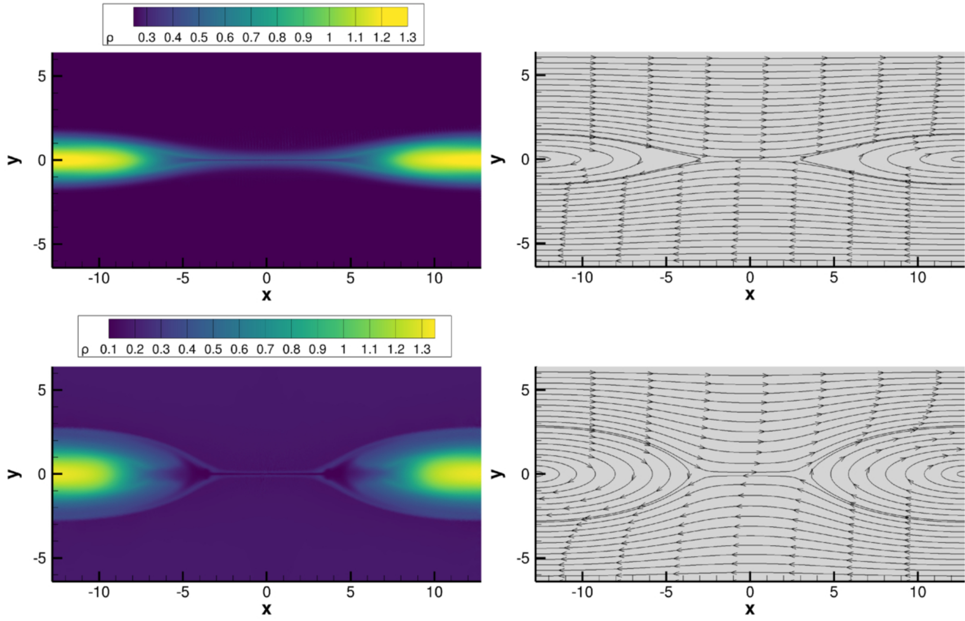
Figure 8. from Rayan Dhib et al 2026 Astrophys. J. Suppl. 283 doi:10.3847/1538-4365/ae4ec1 https://dx.doi.org/10.3847/1538-4365/ae4ec1 © 2026. The Author(s). Published by the American Astronomical Society.
