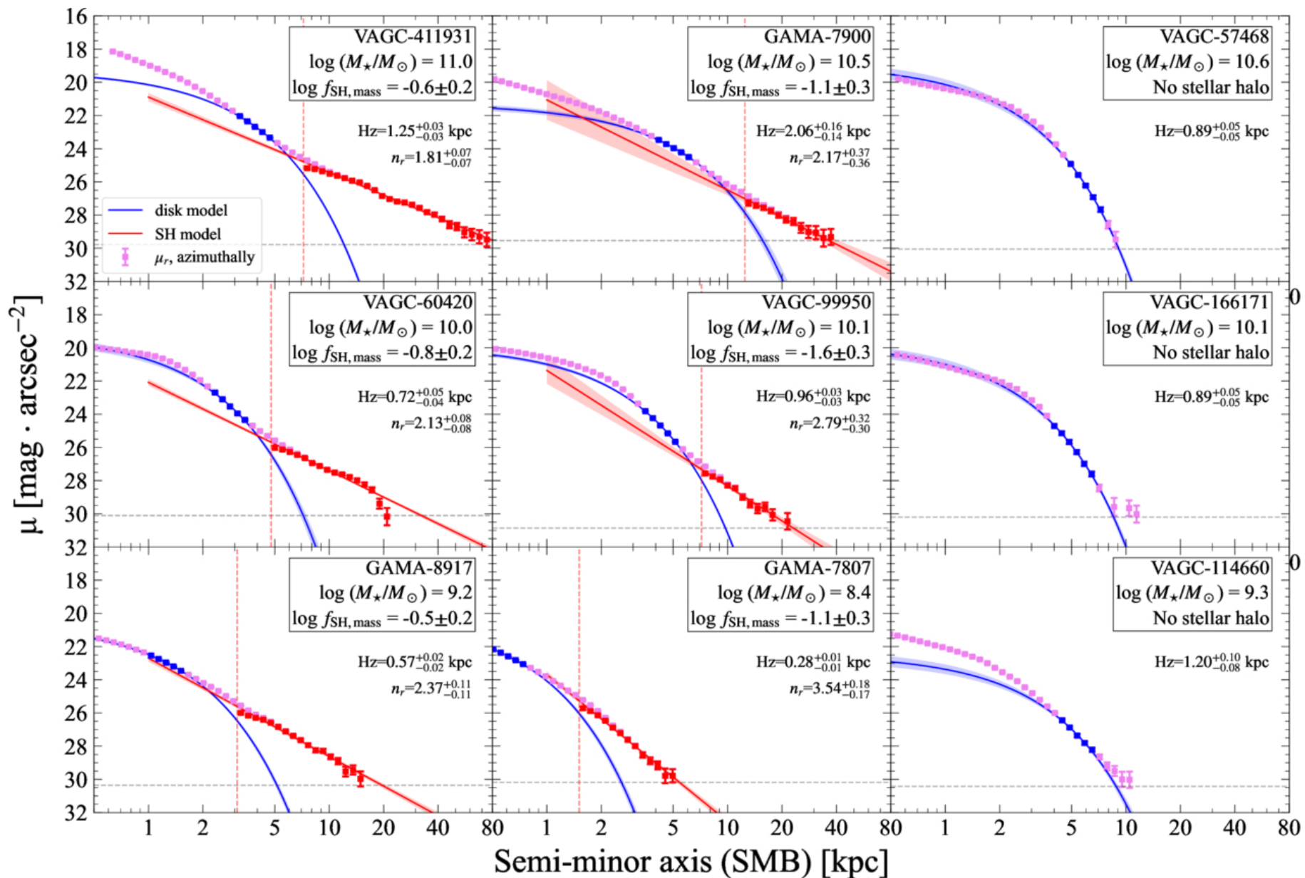
Figure 8. from Bojun Tao et al 2026 Astrophys. J. Suppl. 284 doi:10.3847/1538-4365/ae48ec https://dx.doi.org/10.3847/1538-4365/ae48ec © 2026. The Author(s). Published by the American Astronomical Society.
