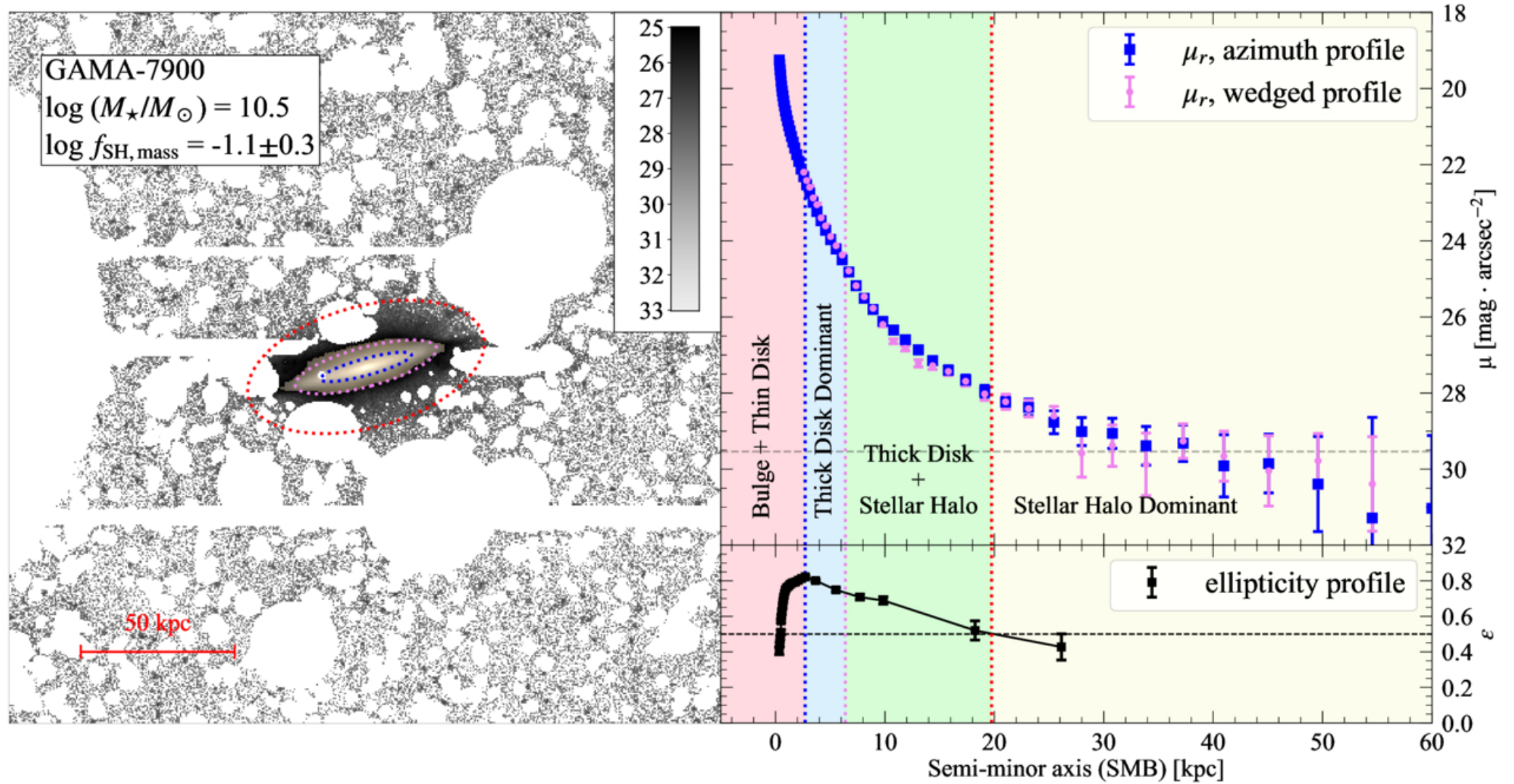
Figure 7. from Bojun Tao et al 2026 Astrophys. J. Suppl. 284 doi:10.3847/1538-4365/ae48ec https://dx.doi.org/10.3847/1538-4365/ae48ec © 2026. The Author(s). Published by the American Astronomical Society.
