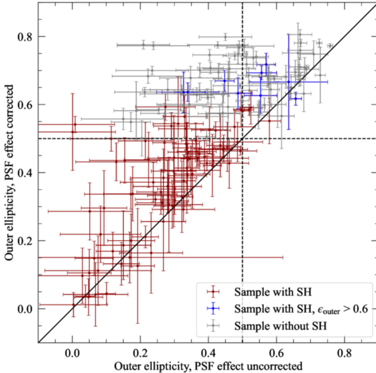
Figure 5. from Bojun Tao et al 2026 Astrophys. J. Suppl. 284 doi:10.3847/1538-4365/ae48ec https://dx.doi.org/10.3847/1538-4365/ae48ec © 2026. The Author(s). Published by the American Astronomical Society.
