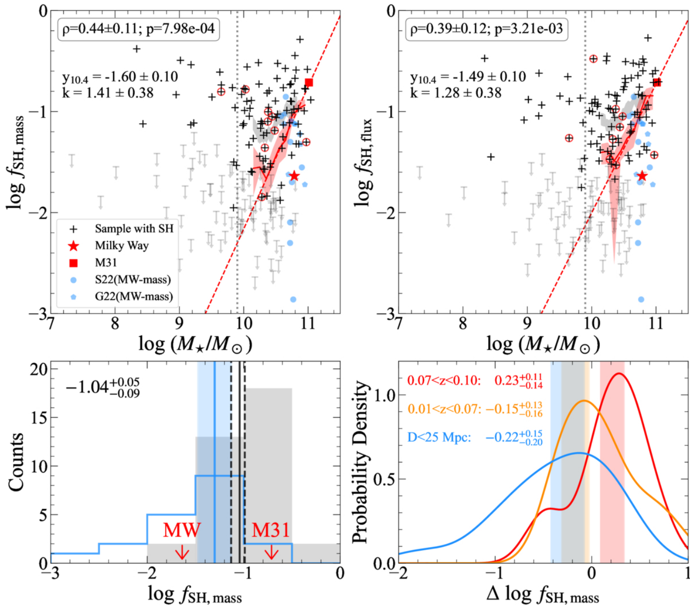
Figure 15. from Bojun Tao et al 2026 Astrophys. J. Suppl. 284 doi:10.3847/1538-4365/ae48ec https://dx.doi.org/10.3847/1538-4365/ae48ec © 2026. The Author(s). Published by the American Astronomical Society.
