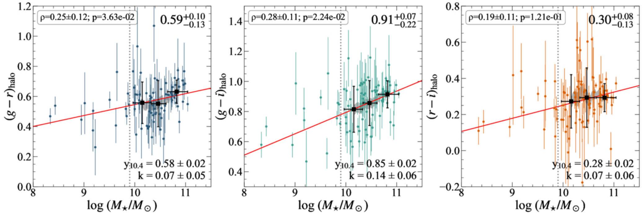
Figure 12. from Bojun Tao et al 2026 Astrophys. J. Suppl. 284 doi:10.3847/1538-4365/ae48ec https://dx.doi.org/10.3847/1538-4365/ae48ec © 2026. The Author(s). Published by the American Astronomical Society.
