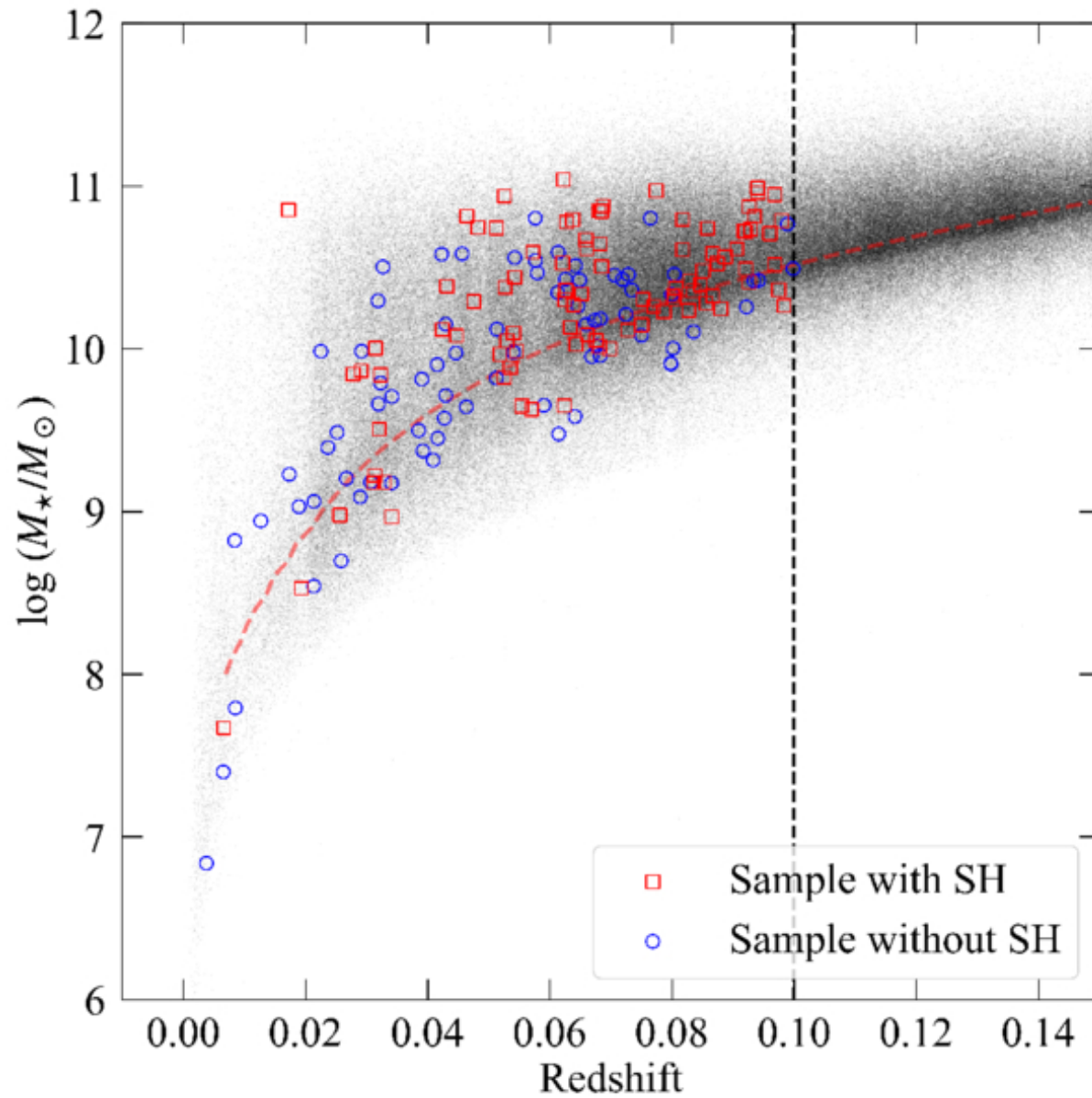
Figure 1. from Bojun Tao et al 2026 Astrophys. J. Suppl. 284 doi:10.3847/1538-4365/ae48ec https://dx.doi.org/10.3847/1538-4365/ae48ec © 2026. The Author(s). Published by the American Astronomical Society.
