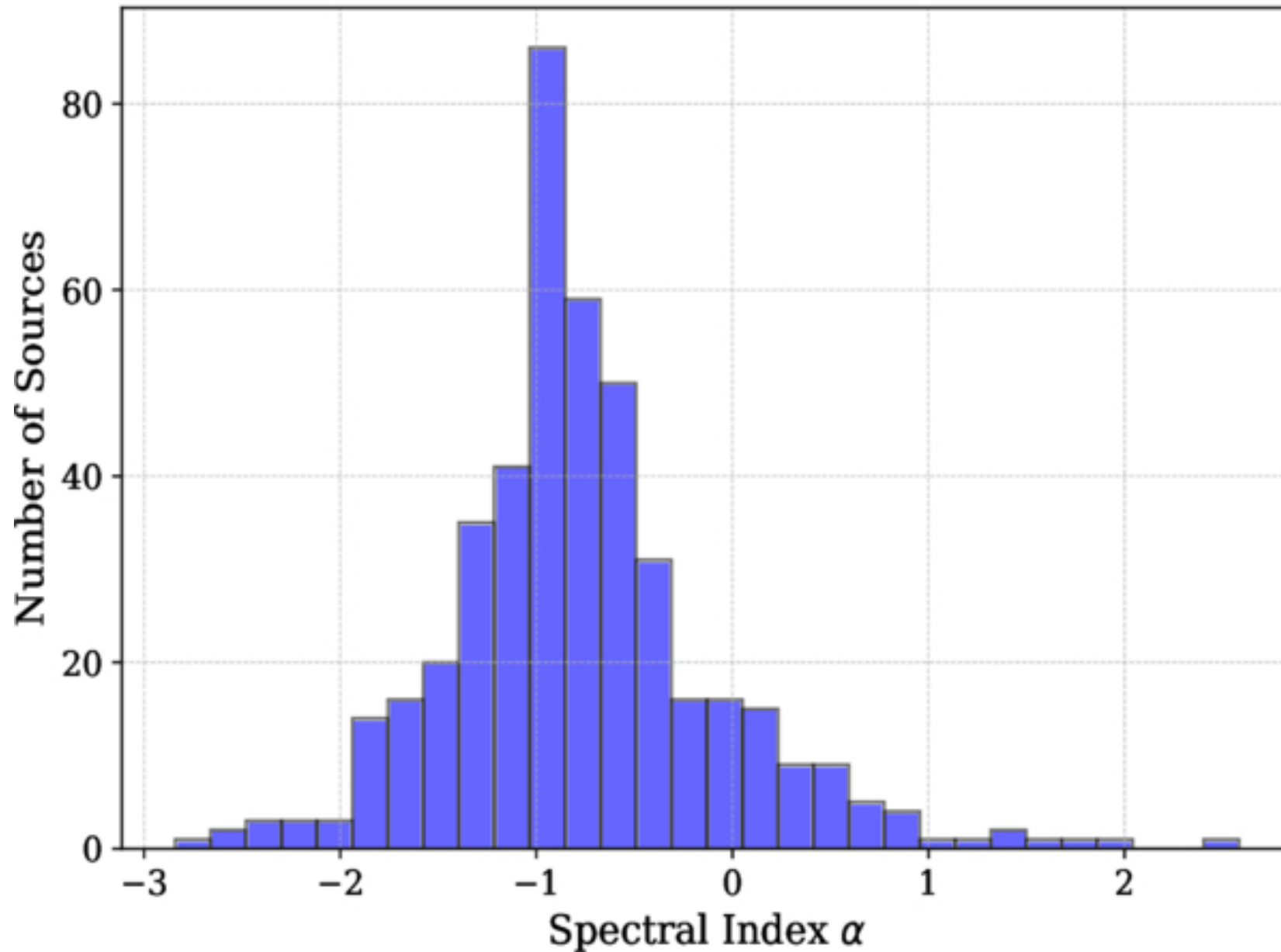
Figure 9. from Haleh Hajizadeh et al 2026 Astrophys. J. Suppl. 283 doi:10.3847/1538-4365/ae472e https://dx.doi.org/10.3847/1538-4365/ae472e © 2026. The Author(s). Published by the American Astronomical Society.
