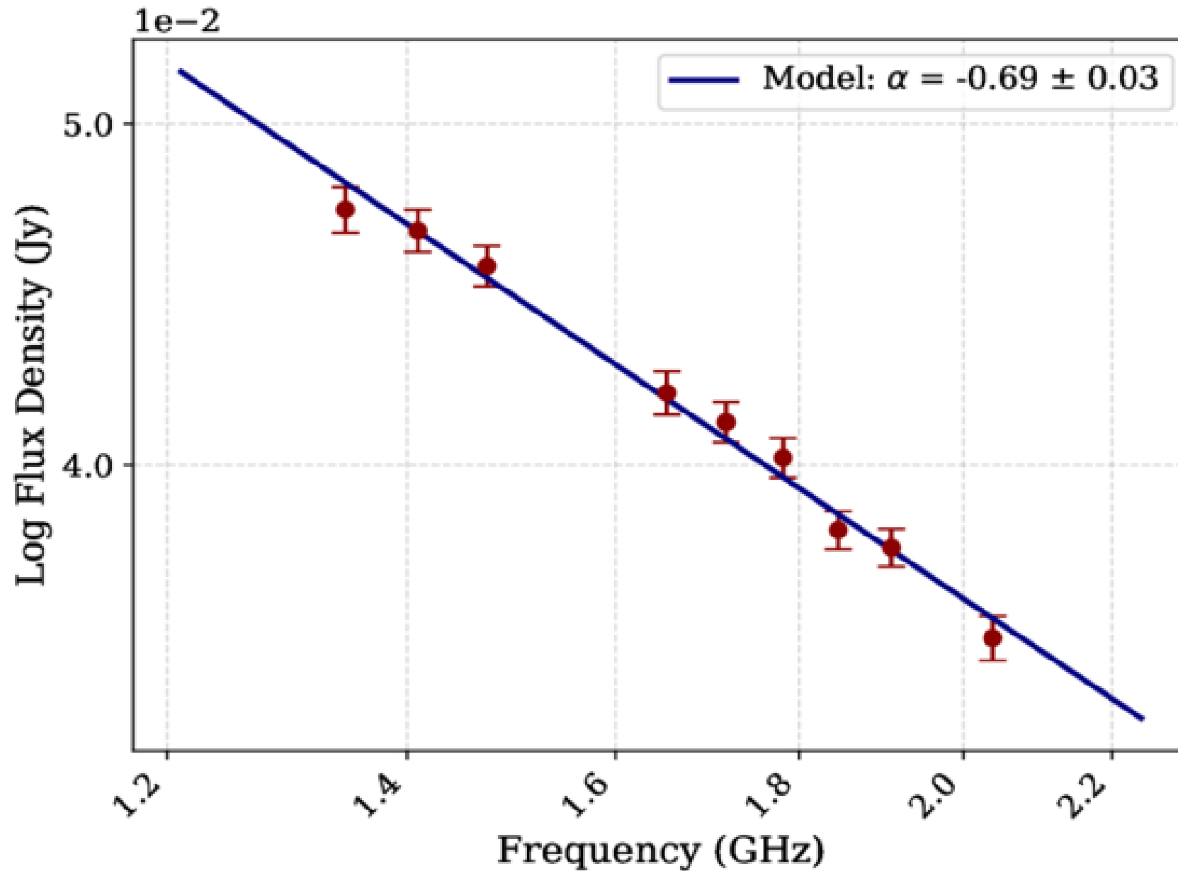
Figure 8. from Haleh Hajizadeh et al 2026 Astrophys. J. Suppl. 283 doi:10.3847/1538-4365/ae472e https://dx.doi.org/10.3847/1538-4365/ae472e © 2026. The Author(s). Published by the American Astronomical Society.
