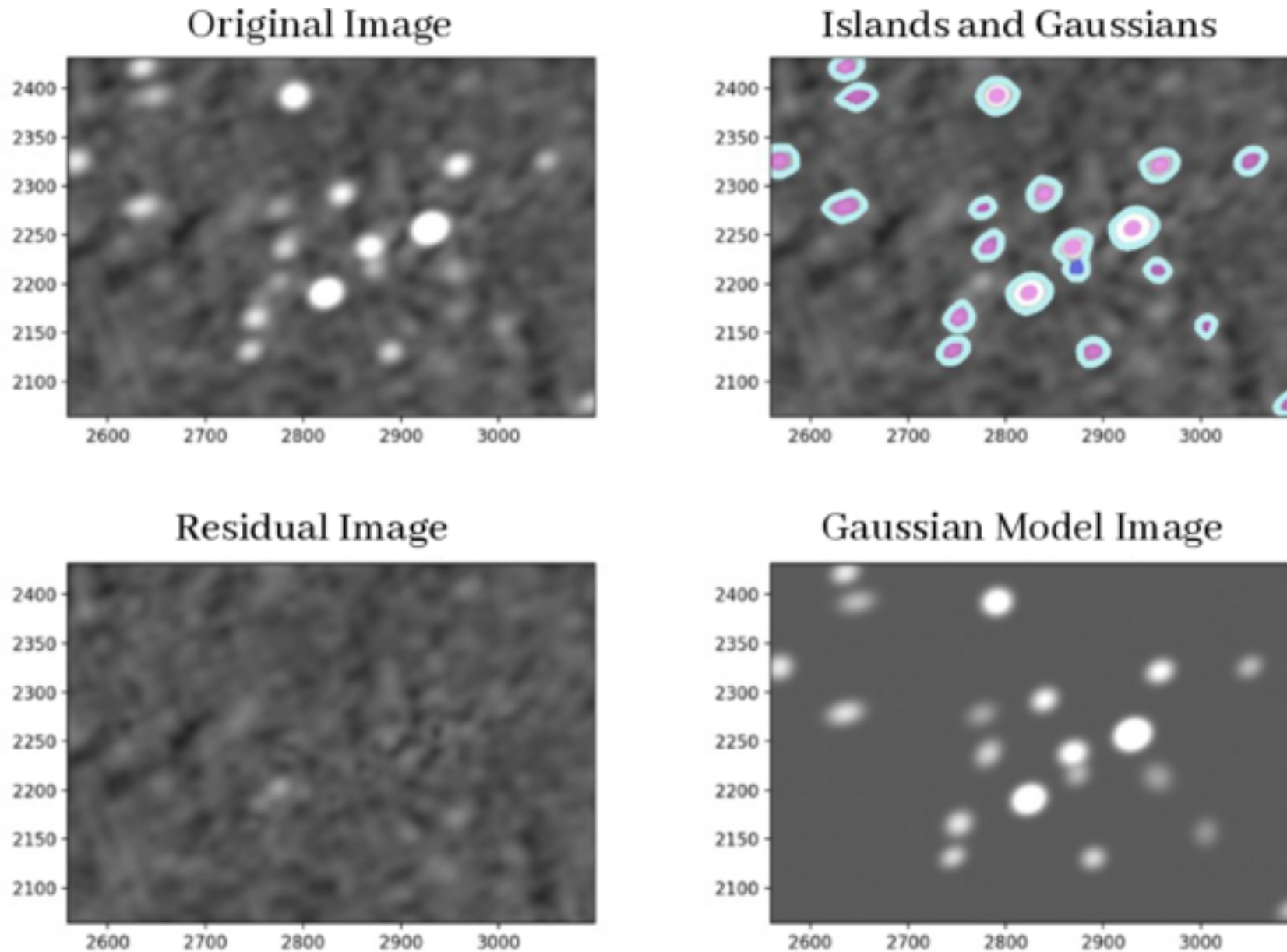
Figure 4. from Haleh Hajizadeh et al 2026 Astrophys. J. Suppl. 283 doi:10.3847/1538-4365/ae472e https://dx.doi.org/10.3847/1538-4365/ae472e © 2026. The Author(s). Published by the American Astronomical Society.
