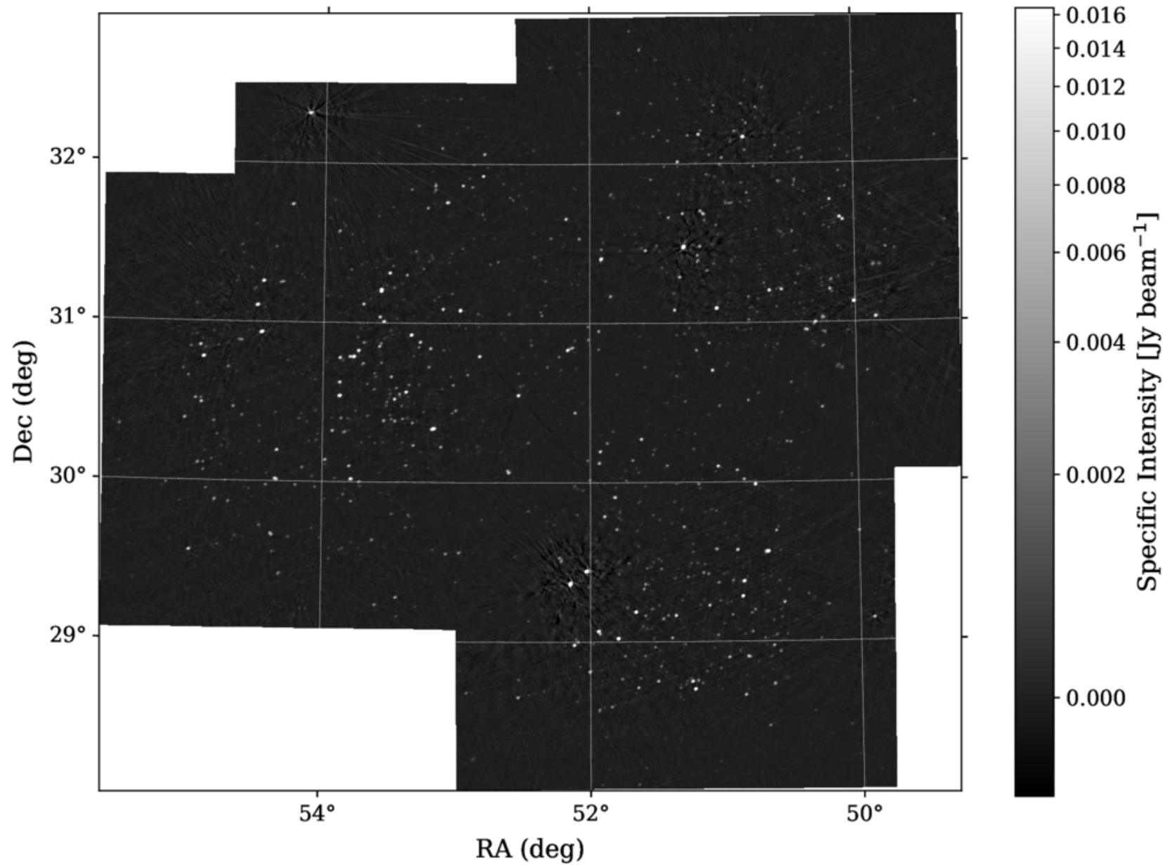
Figure 2. from Haleh Hajizadeh et al 2026 Astrophys. J. Suppl. 283 doi:10.3847/1538-4365/ae472e https://dx.doi.org/10.3847/1538-4365/ae472e © 2026. The Author(s). Published by the American Astronomical Society.
